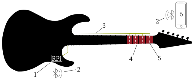
Figure 2: Schematic of Let's Frets . A Raspberry Pi (1) communicates via Bluetooth (2) with a smartphone app (6). The conductive frets (4) and LEDs (5) are connected via cables to the Raspberry Pi.
